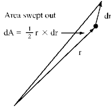
Fig. 9.1 The radius vector \mathbf{r} of a particle with angular momentum \mathbf{L} = m\mathbf{r} \times d\mathbf{r}/dt sweeps out a vector area d\mathbf{A} = (\mathbf{L}/2m)dt in time dt .
