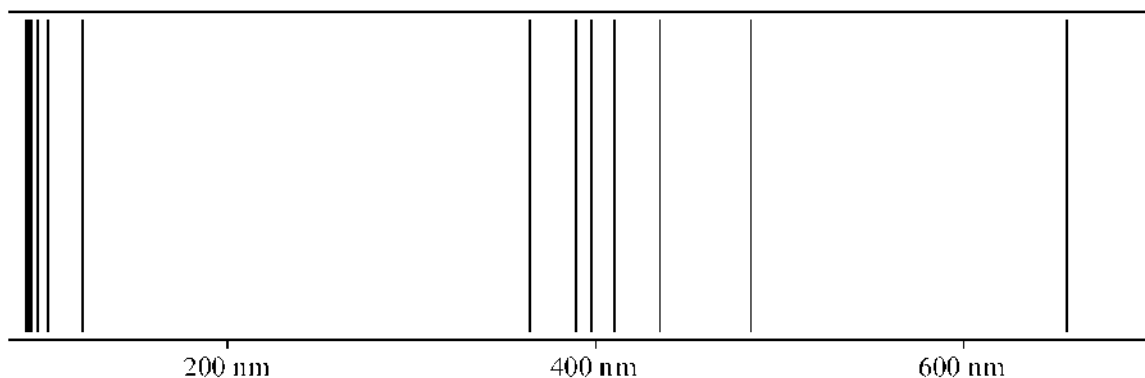
Fig. 1.5 Spectral lines of atomic hydrogen. The series of lines in the visible part of the electromagnetic spectrum, called the Balmer series , arises from transitions between states with principal quantum number n = 3, 4, 5, \dots and a state with n = 2 . The series of lines in the ultraviolet, called the Lyman series , arises from transitions between states with principal quantum number n = 2, 3, \dots and the ground state with n = 1 .
